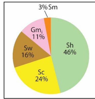
Upper shoreface
