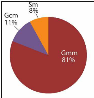
Gravity-flow-deposits
