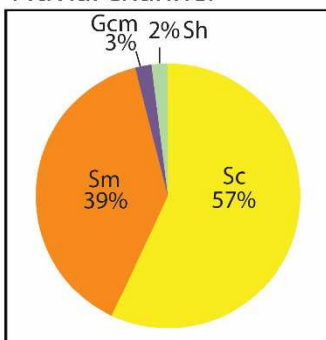
Fluvial channel
