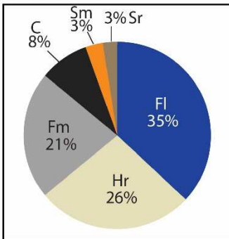
Overbank
