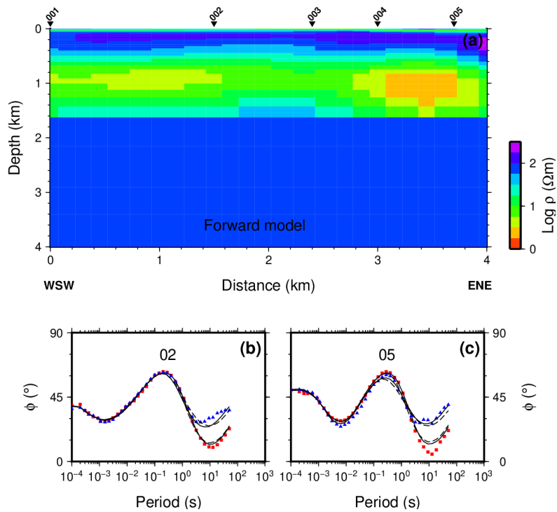
Figure A2. Sensitivity test using forward modeling to check if the variation in the depth of the resistive basement is a required feature in the inversion model of Fig. 9. (a) Section of the edited geoelectric model; (b) comparison between the experimental phases (square symbols for TE mode and triangle symbols for TM mode) with phases from the inversion (continuous lines) and edited (dashed lines) models at site 02; (c) the same as (b) at site 05.
