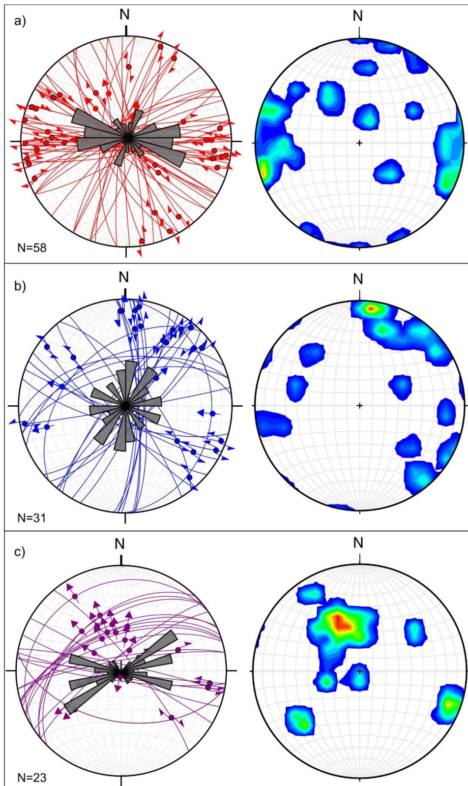
Supplementary figure A2. Kinematic data (Schmidt diagram, lower hemisphere) from the major fault zone domains of the Cinzas Catchment; great circles, rose diagrams and poles of surfaces of a) right-lateral strike-slip faults, b) left-lateral strike-slip faults and c) normal faults.
